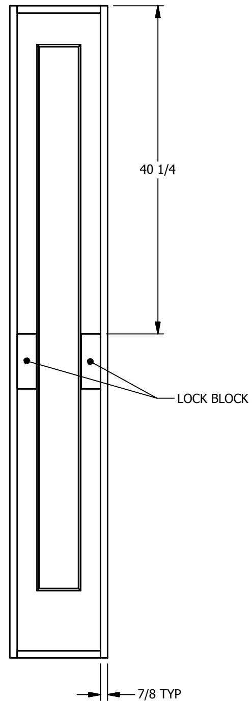
LOCK BLOCK LOCATION DOOR SKIN REMOVED
